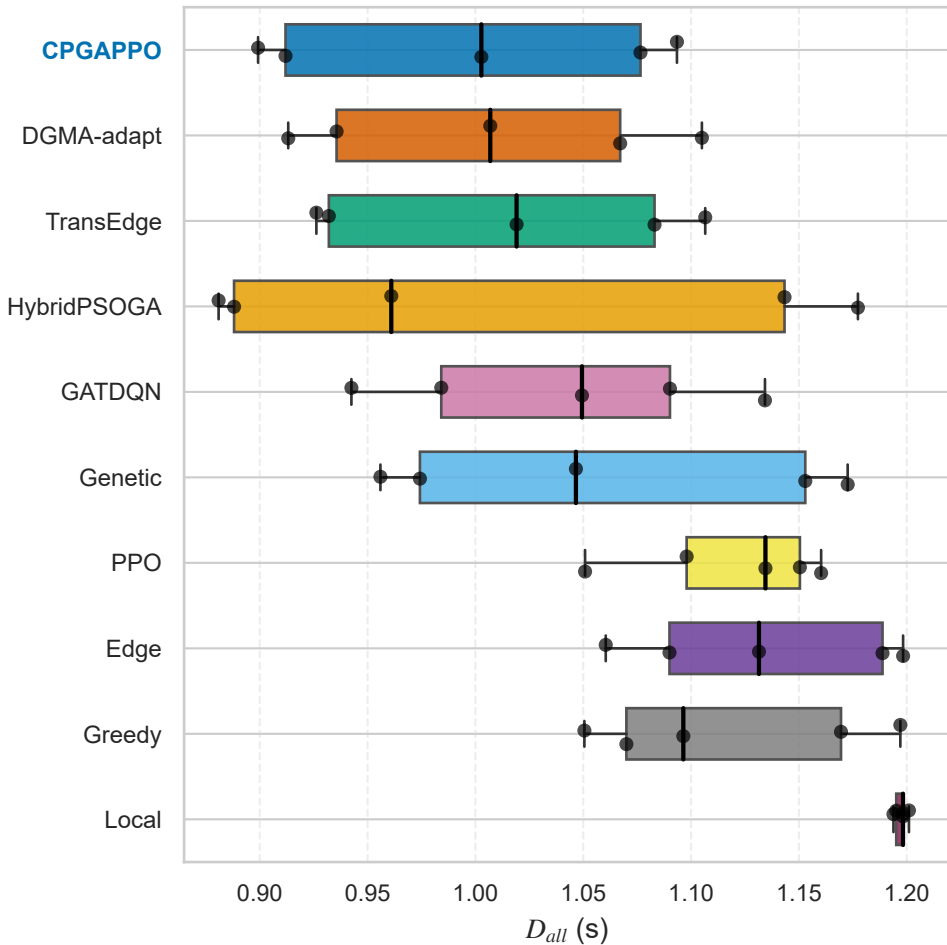
All-app latency D_{all} (per-seed cross-DAG avg, median + IQR, n=5 seeds)
